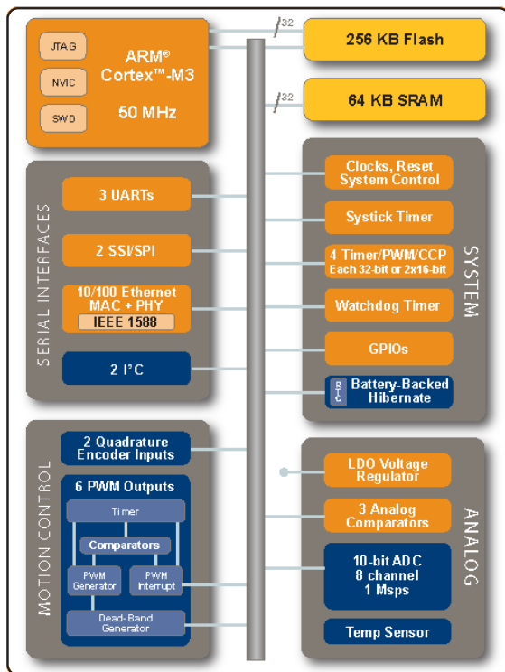
LM3S6000 Series Block Diagram. This block diagram shows the superset of features for the LM3S6000 series of microcontrollers.
